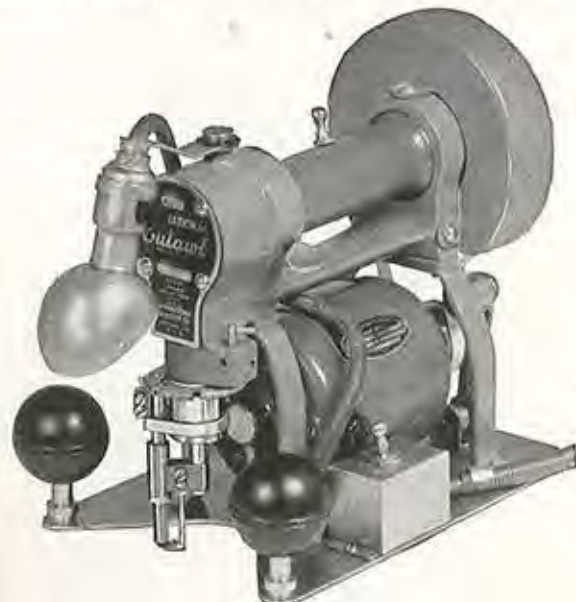
Figure 1—The K9 Cutawl
