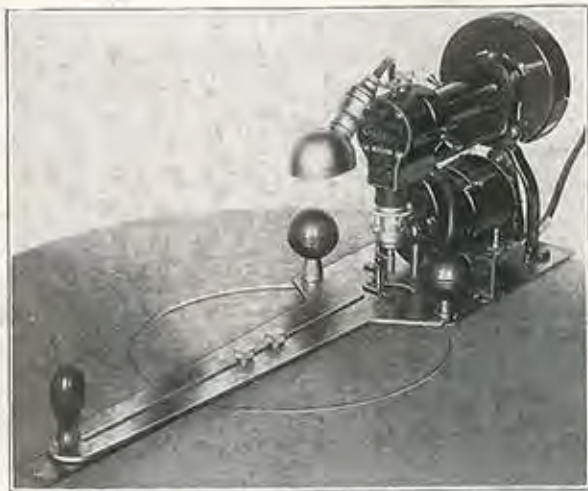
Figure 17—Circle Cutting Attachment
